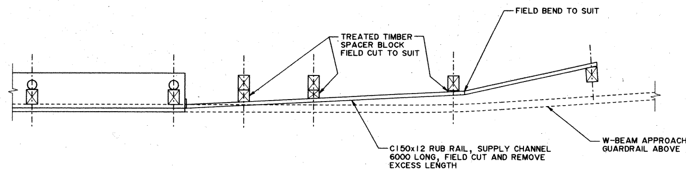
PLAN - CHANNEL RUB RAIL 1:25
