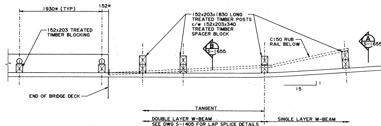
PLAN - W-BEAM GUARDRAIL 1:25
