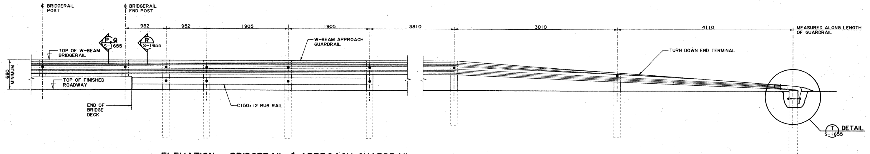
ELEVATION - BRIDGERAIL & APPROACH GUARDRAIL 1:25
